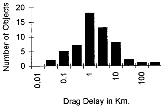
One Day Drag Retardation for Typical 300-600 km. Objects
