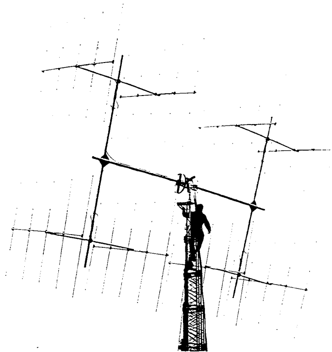
Figure 1. The VHF Ionization Radar Antenna System
