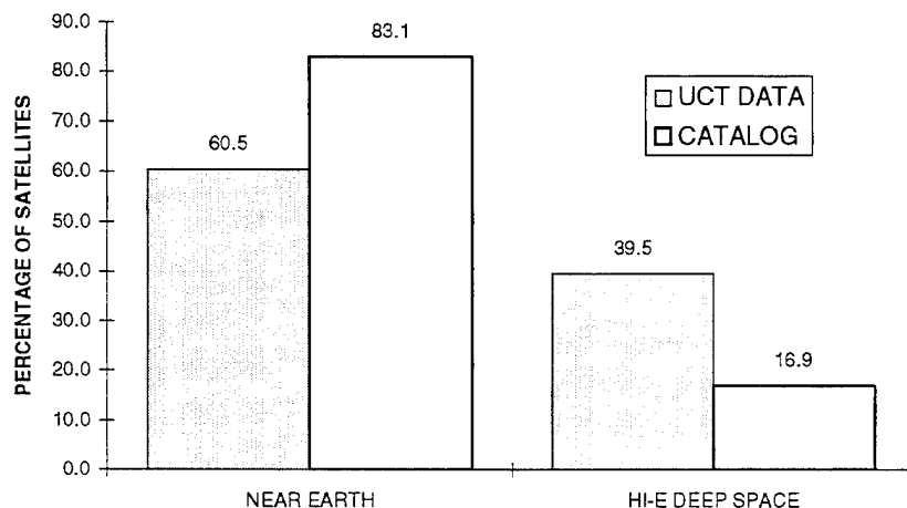
Population Distribution Figure 1
