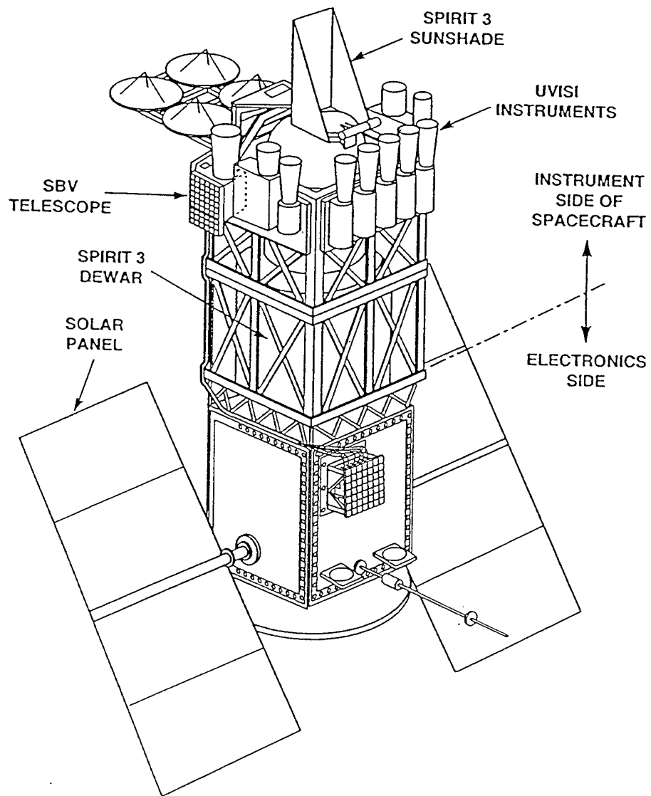
Figure 1. MSX satellite
