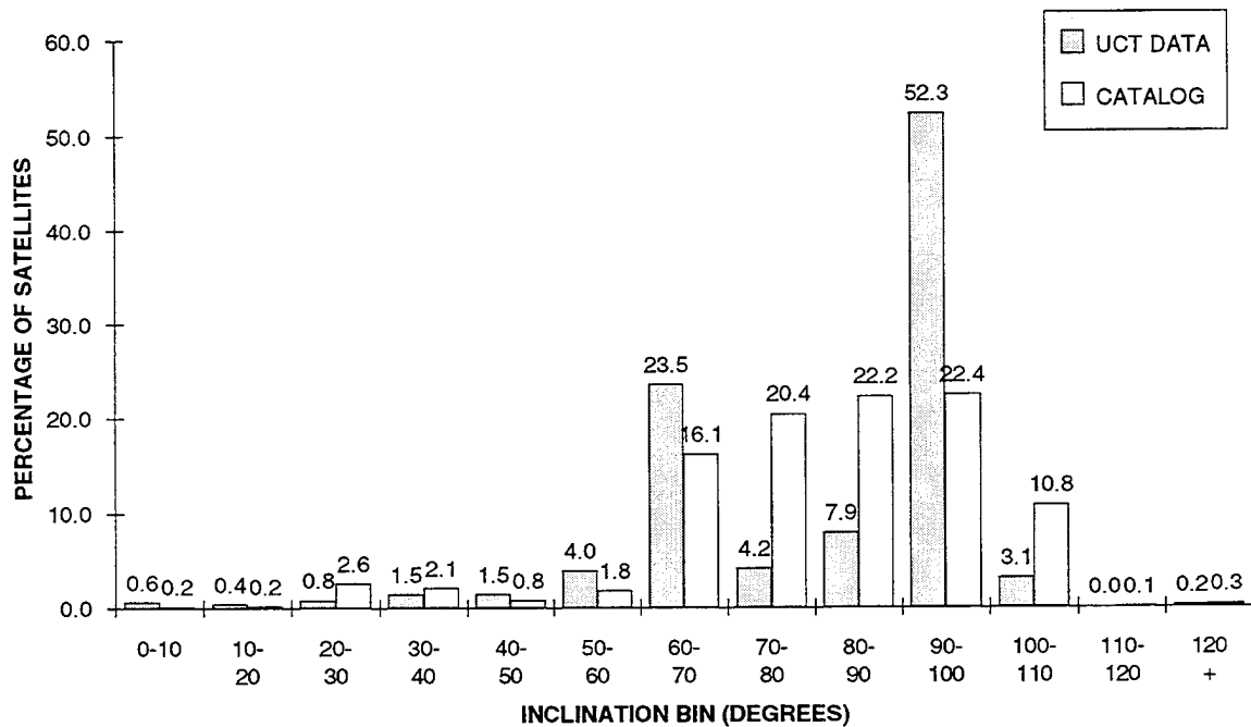
Near Earth Inclination Distribution Figure 3
