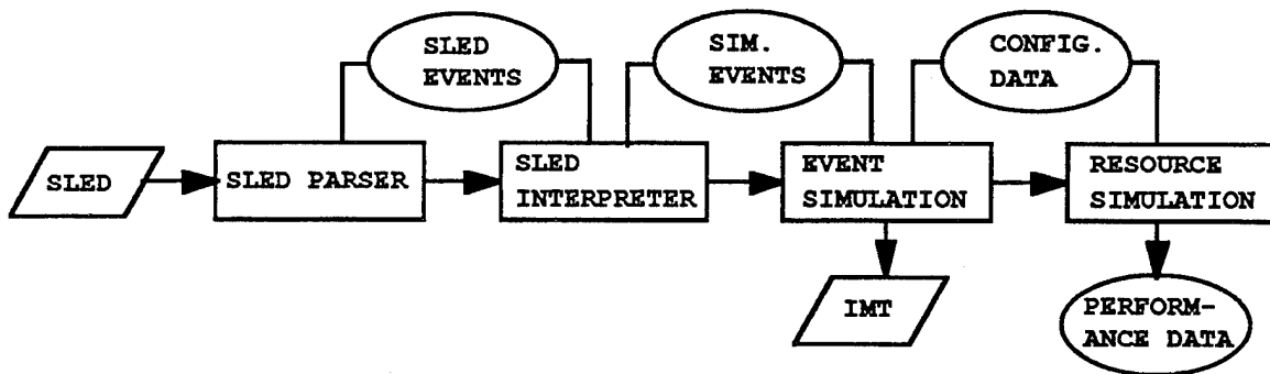
Figure 8. Simulator Architecture
