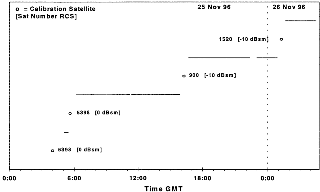
Figure 1. Haystack 24-Hour Measurement Campaign Time Line
