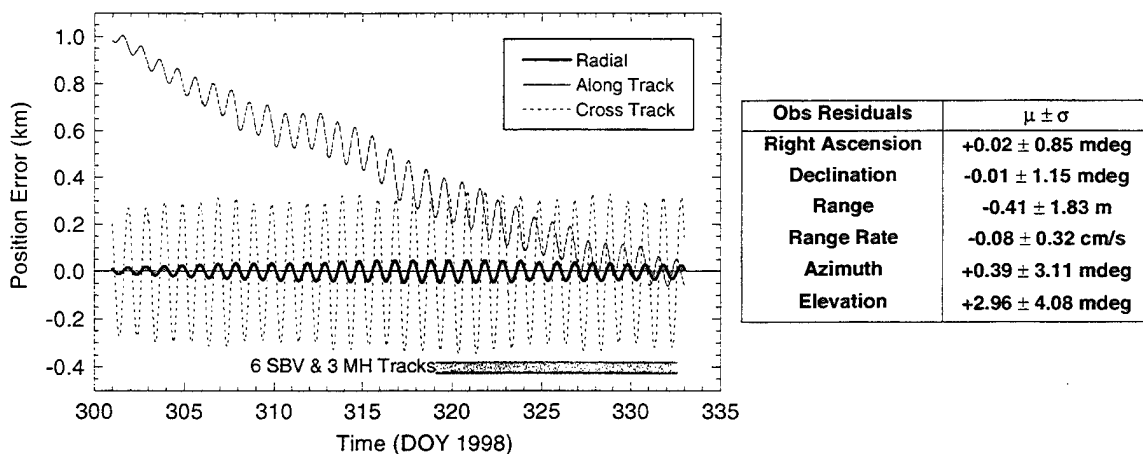
Figure 8. Two week SBV and Millstone tracking orbit comparison
