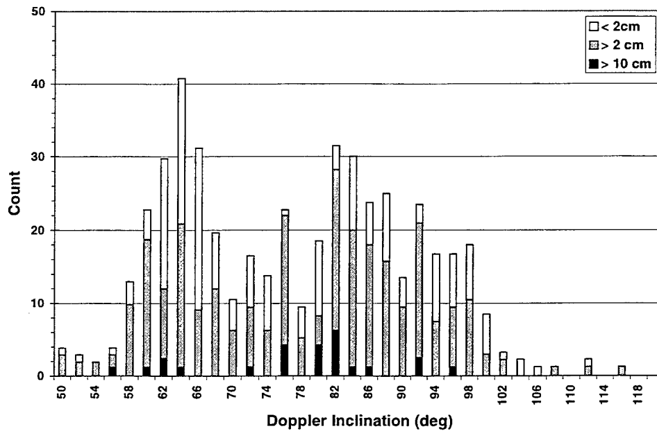
Figure 13. TIRA/EFPE, Inclination Distribution for Altitude 600 - 1200 km
