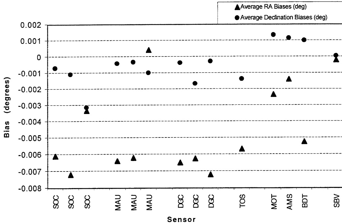
Figure 9. Average Biases of Optical Sensors for 1998
