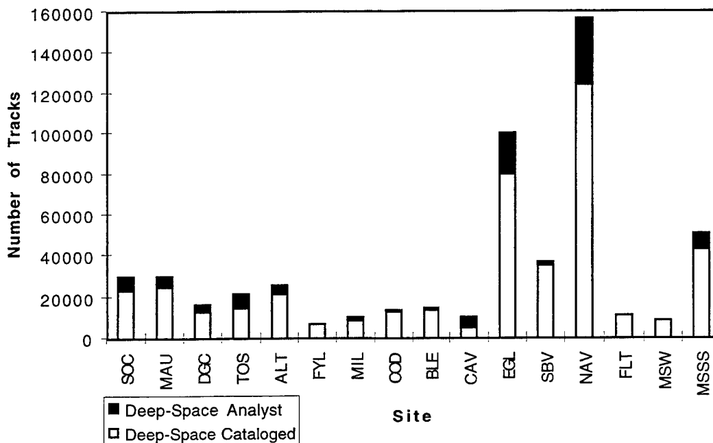
Figure 4. Tracks on Deep-Space Satellites from 13 April through 31 December 1998
