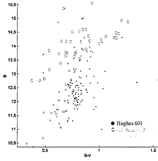
Figure 4. Color-Magnitude Plot
