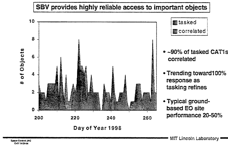
Figure 15. SBV's Category 1 Tracking Performance
