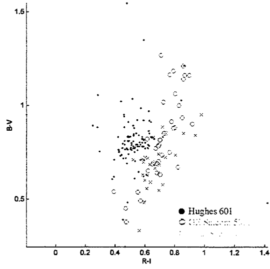
Figure 5. Color-Color Plot
