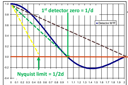
Nyquist Optics MTF
